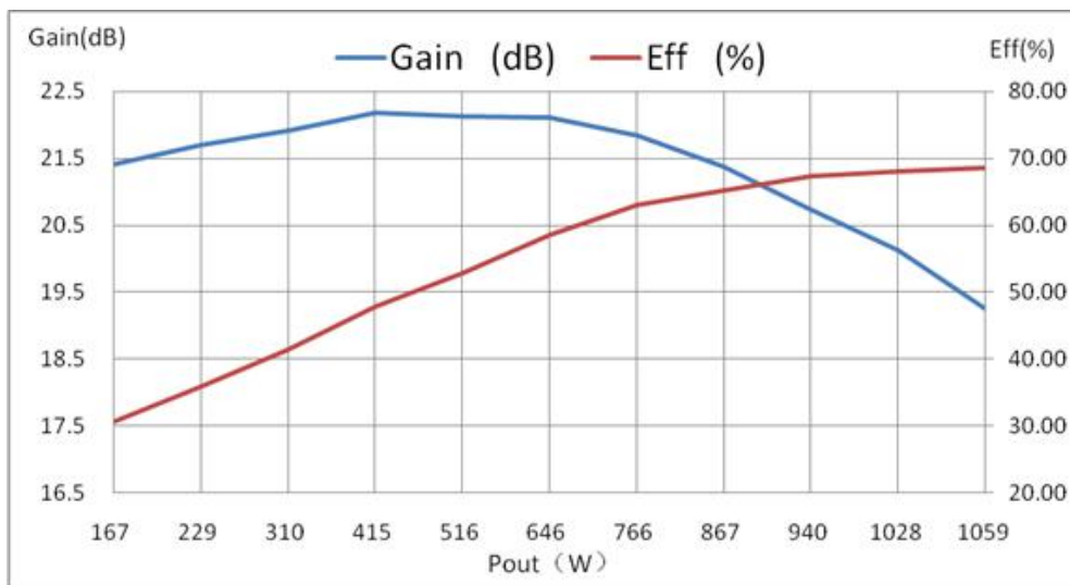
Figure 1: 440MHz Pulsed CW gain and efficiency as a Function of Output Power
